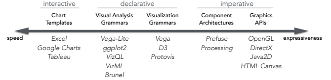
Figure 1: Axis of visualization specification. Data visualizations are created with a spectrum of tools with a spectrum of speed and expressivity. Some of these tools are faster but others are more expressive to create visualizations.
